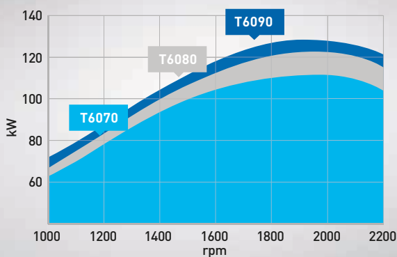
Power Curves
