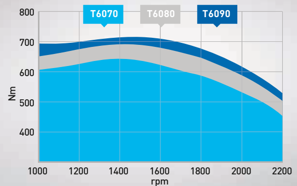
Torque Curves
