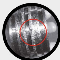
DAMAGE TO THE PUMP PISTON
