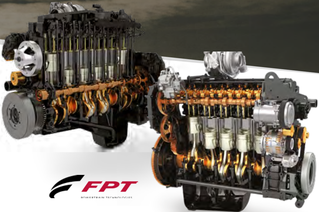
◀ 8.7L engine
