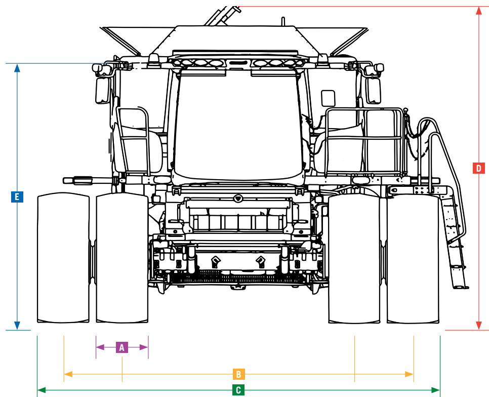
250 SERIES DIMENSIONS
