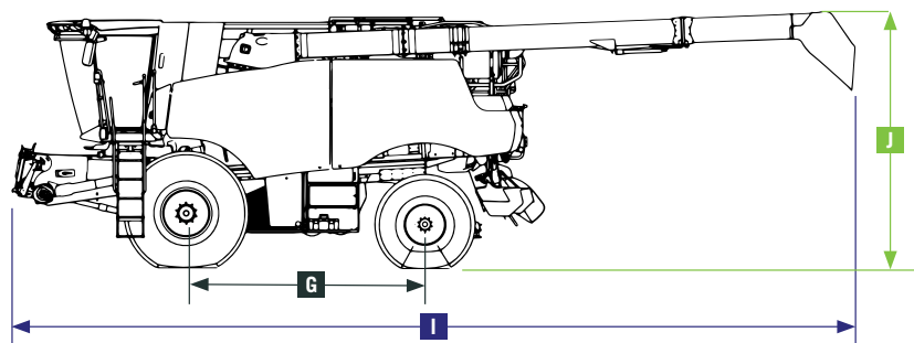
250 SERIES DIMENSIONS
