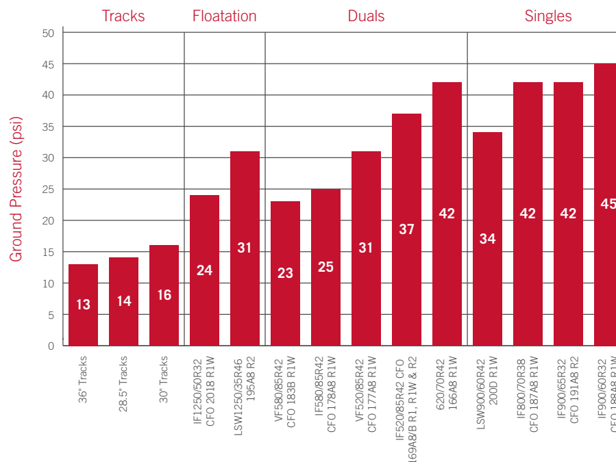
8250 GROUND PRESSURE COMPARISON (2022 COMBINE MODEL)
