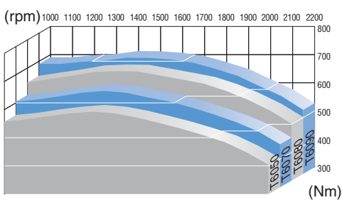
Torque Curves
